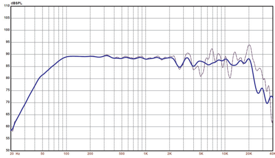
Figure1: SPL on axis (dotted) and reference angle 10°
