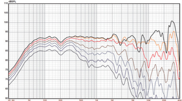
Figure2: SPL from 0° to 90°
