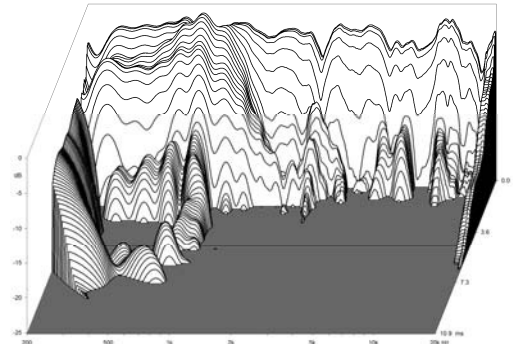
Figure4: Cumulative spectral decay
